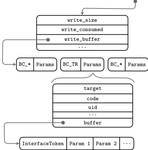
Figure 3: Parameters of a BINDER_WRITE_READ ioctl.
